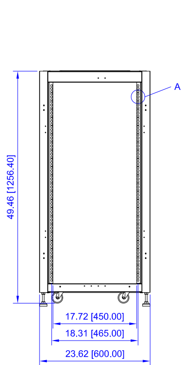
FRONT VIEW (NO DOOR)
