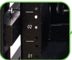
Mounting rails, complete with 10-32 tapped holes and easy to read RU markings
