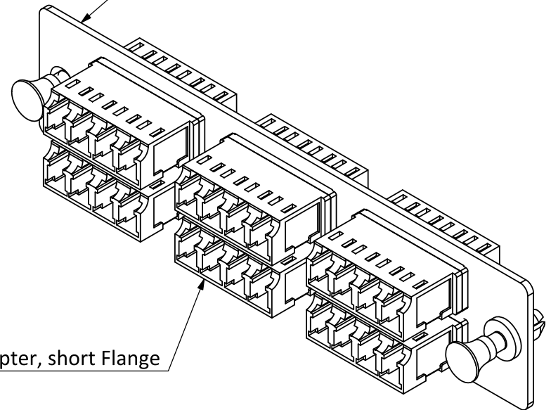
LGX Fiber Adapter Panel
