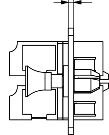
LGX Fiber Adapter Panel
