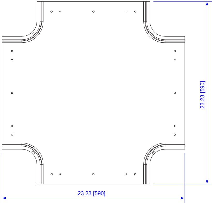
TOP VIEW
