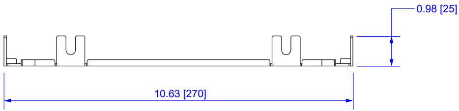
TOP VIEW
